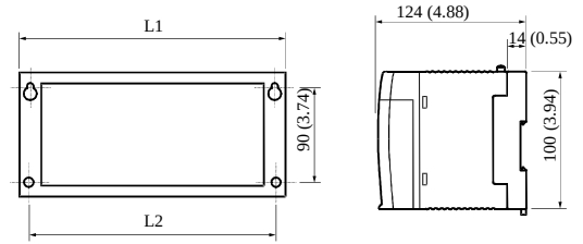
Figure 11.2 External dimensions
