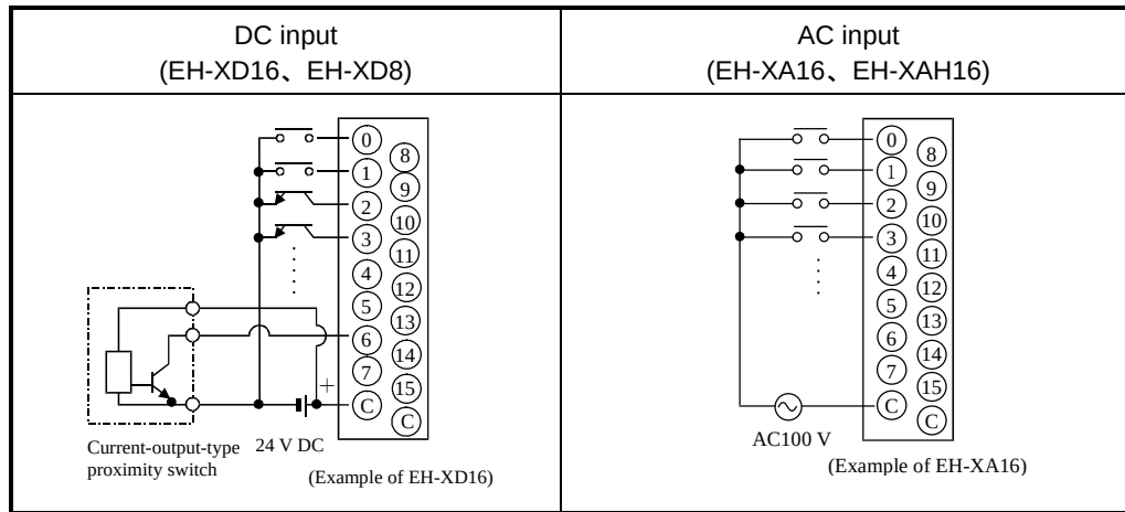
Figure 11.5 Input wiring
