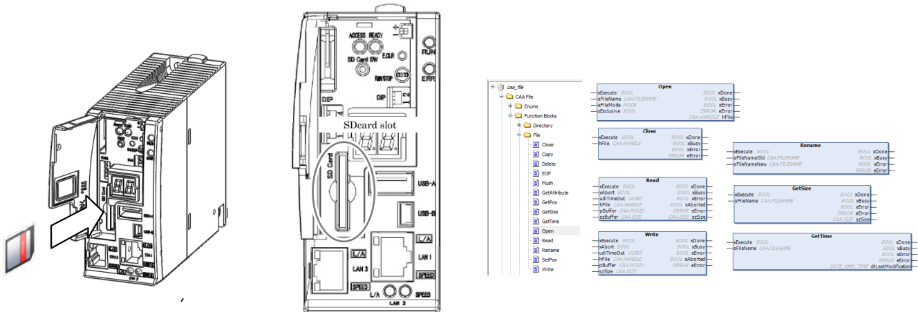
Figure 4.5 SD card
